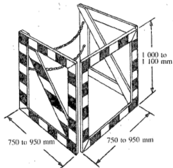
Wooden guardrail, Fig. 2 ss
