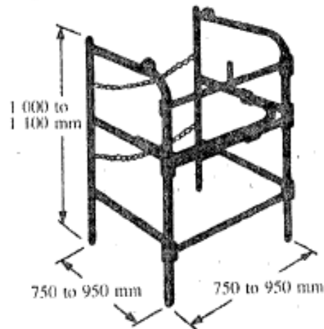
Steel guardrail, Fig. 1
