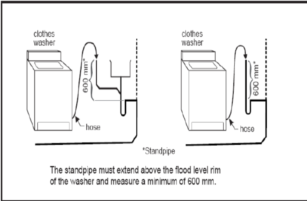
Figure A-2.4.9.3.(3) Standpipe Illustration
