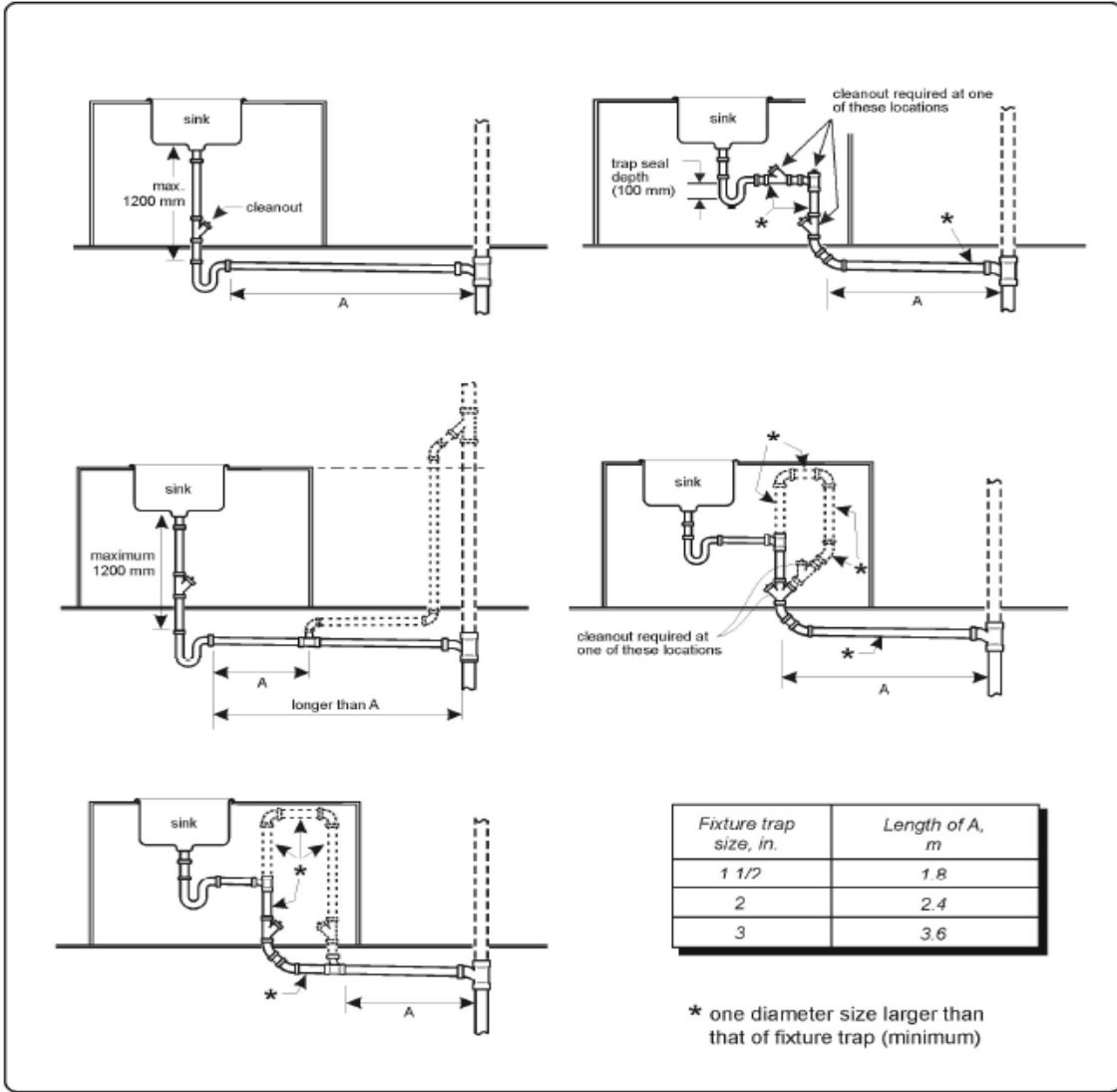
Figure A-2.4.8.2.(1) Island Fixture Installation.
